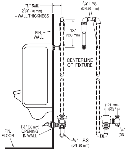
Model 323 — Water Saver (1.5 gpf/5.7 Lpf) Model 323-1.0 Low Consumption (1.0 gpf/3.8 Lpf)
