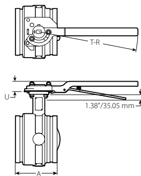
VALVE WITH LEVER LOCK HANDLE AND MEMORY STOP 8”/200 MM SIZES
