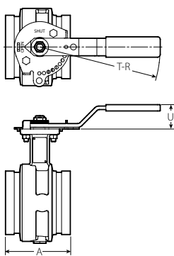
10-POSITION HANDLE WITH MEMORY STOP 2 – 6”/50 – 150 MM SIZES
